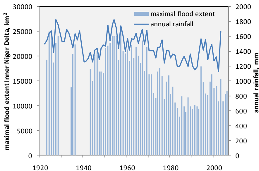
Figure 5-4- The flood extent of the Inner Niger Delta (columns; left-handed axis) and annual rainfall in the Upper Basin of the Niger (based on data given in Figs. 9 and 10) (line; right-hand axis).
