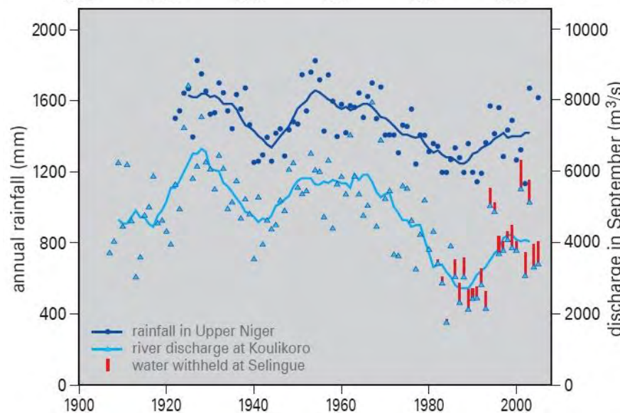
Figure 3-5- Annual rainfall of the Upper Niger (dark blue symbols, left y-axis) averaged for 17 rainfall stations in the catchment area, and the river discharge in September in Koulikoro (light blue symbols, right y-axis). The trends show 9-year running means. The red bars show the effect of the Sélingué reservoir on the river discharge in September. See Fig. 3.3 for the location of Sélingué, Koulikoro and the rainfall stations. From: Zwarts et al. (2009).
