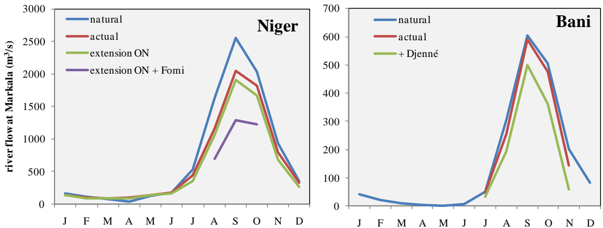
Figure 4-2- The natural, actual and future monthly flow of the Niger River at Markala (downstream of the dam) (left) and of the Bani River at Sofara (right). All data from Table 4.4 for the Niger and from Table 4.7 for the Bani.
