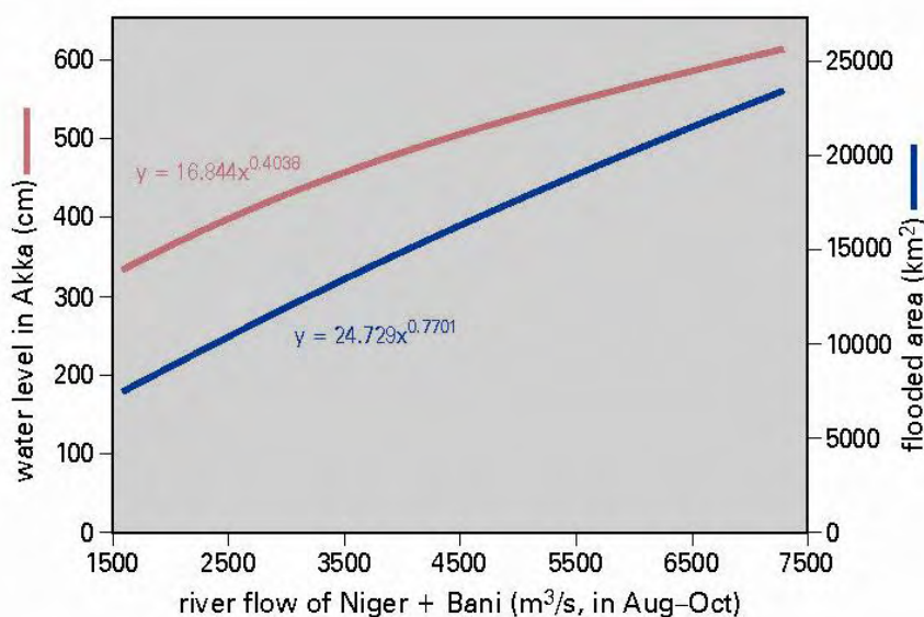
Figure 5-3- The highest water level in Akka (cm; red line, left axis) reached within a year as a function of the combined river discharge of the Niger (downstream of the Markala dam) and the Bani (Douna), averaged for August-October that year. The blue line gives the same relationship for the flooded surface (km 2 ). From: Zwarts & Grigoras (2005).
