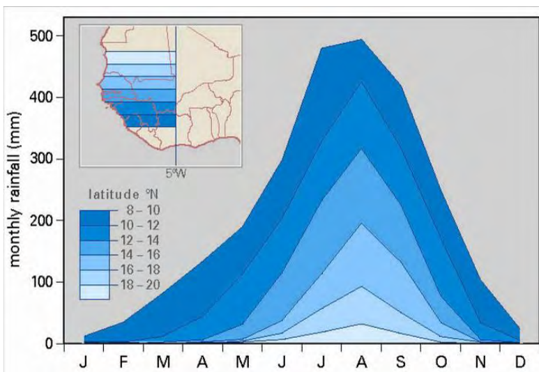
Figure 3-2 - The average monthly rainfall in West Africa (west of 5° given per latitude; the countries are indicated. The rainfall given for 14-16°N and 12-14°N refers to the northern and southern Inner Niger Delta, respectively. There is more rain in the southern Delta (as already shown in Fig. 3.1), but the raining season also extends over a longer period as in the northern Delta. The raining season starts still earlier in the headwaters of the Niger (8-12°N). From: Zwartz et al. (2009).
