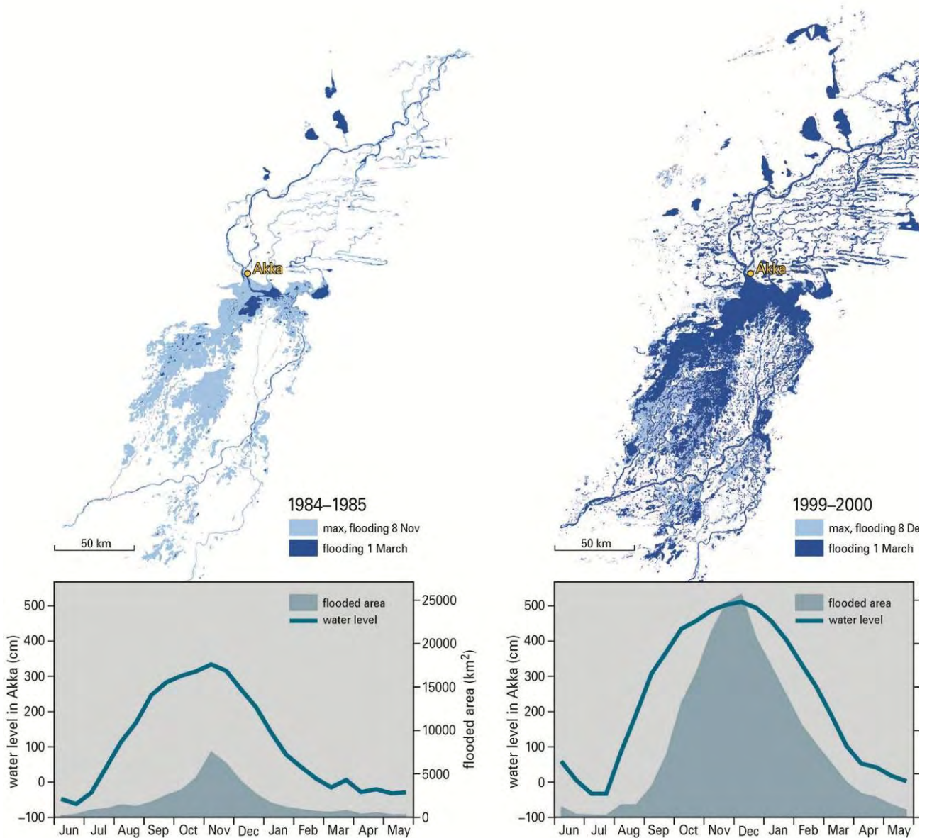
Figure 5-2- The graphs show daily measurements of the water level at Akka (left axis in both graphs) between June and May in 1984/85 (left graph; the lowest flood ever measured) and in 1999/2000 (right graph; one of the highest floods since 1970, but of normal height when compared with pre-1973 floods). The surface areas flooded (right axis in both graphs) in 1984/85 and 1999/2000, shaded in the same graph, are derived from the water level data, using the digital elevation models of Zwarts & Grigoras (2005). The maps show the flooded area when the water level at Akka reached its peak, and for 1 March. Note that the peak flood level in 1999 (511 cm) was 1.5 times higher than in 1984 (336 cm), but that the maximal flood extent was nearly 5 times larger. The difference is even larger some months later. The flood extent on 1 March (shown as dark blue on the map) was in 2000 13 times more than in 1985 (right map). From: Zwarts et al. (2009).
