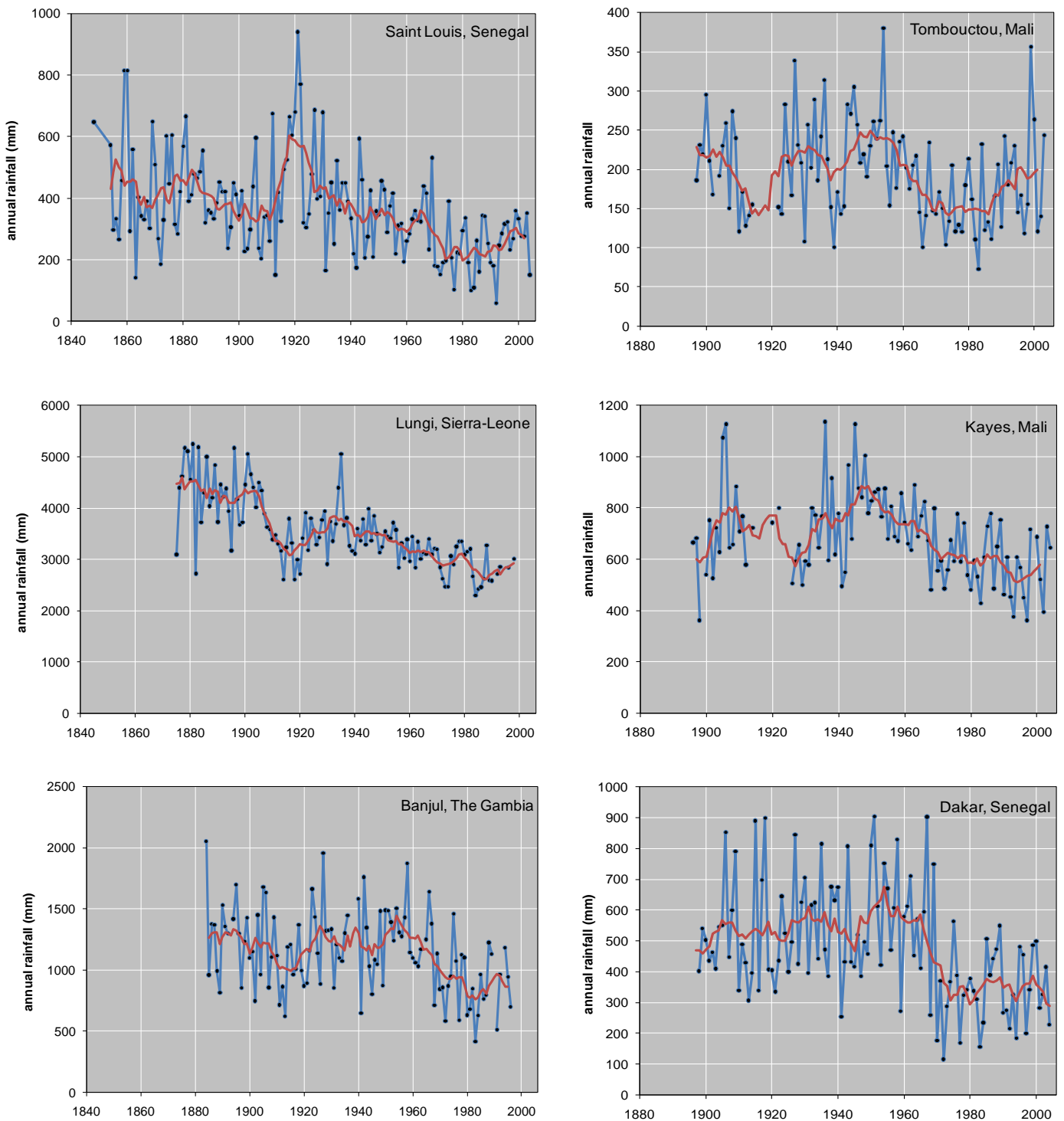
Figure 2-2- The annual rainfall in six meteorological stations in West Africa, having the longest series of measurements (all started before 1900). The red line gives the running mean over an interval of 9 years (4 year before – 4 years after the year concerned)
