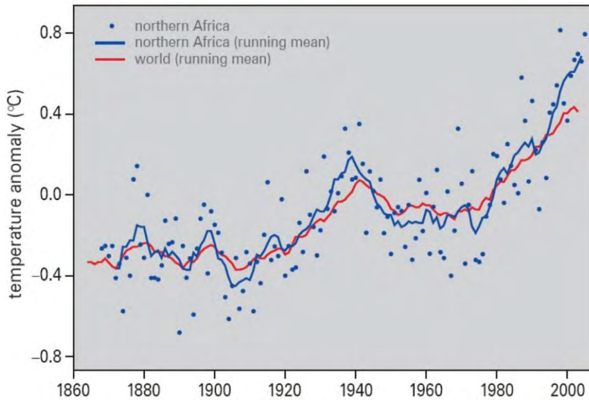
Figure 2-4 - The average temperature given as departures from the 1961-1990 average in northern Africa (0-40°N, 20°W-60°E) and worldwide (source: www.met-office.gov.uk/research/hadleycentre/CR_data/Monthly/HadCRUG.txt ). The trends show the running mean calculated over an interval of 9 years (4 year before – 4 years after the year concerned).
