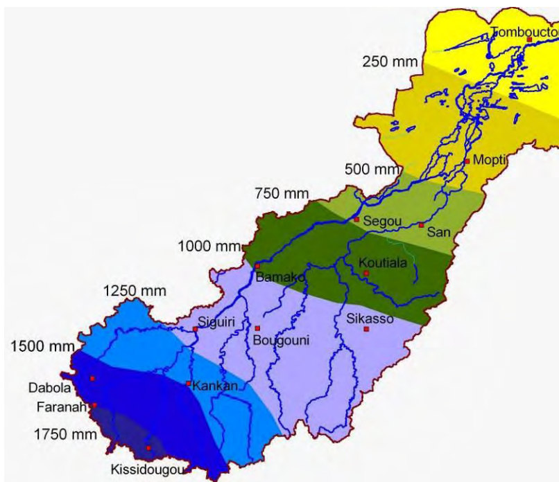
Figure 3-1 - The annual rainfall (mm/year) in the basin of the Upper Niger shown as eight different zones. Thirteen major meteorological stations are indicated with red dots. From: Zwarts et al. (2005).
