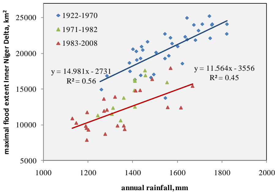
Figure 5-5- The relationship between the flood extent of the Inner Niger Delta and the annual rainfall in the Upper Basin of the Niger; same data as Fig. 5.4. Subdivision into three temporal categories (before 1971 and after 1983 and a between-category) well illustrates how the flood extent has declined due to dams and irrigation schemes, but also due to the increased seepage of surface water (see text and Figs. 9 and 10).
