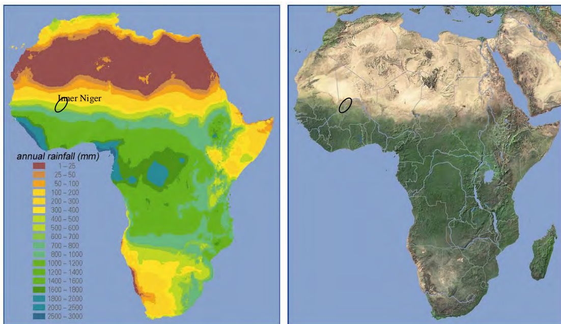
Figure 2-1 - The north of Africa is extremely dry and this holds –to a lesser degree– for the east and southwest. Central Africa, on the contrary, is extremely wet. South of the Sahara the transition from dry to wet south is amazing in its rapidity, with a doubling rainfall for every 160 km southward.
