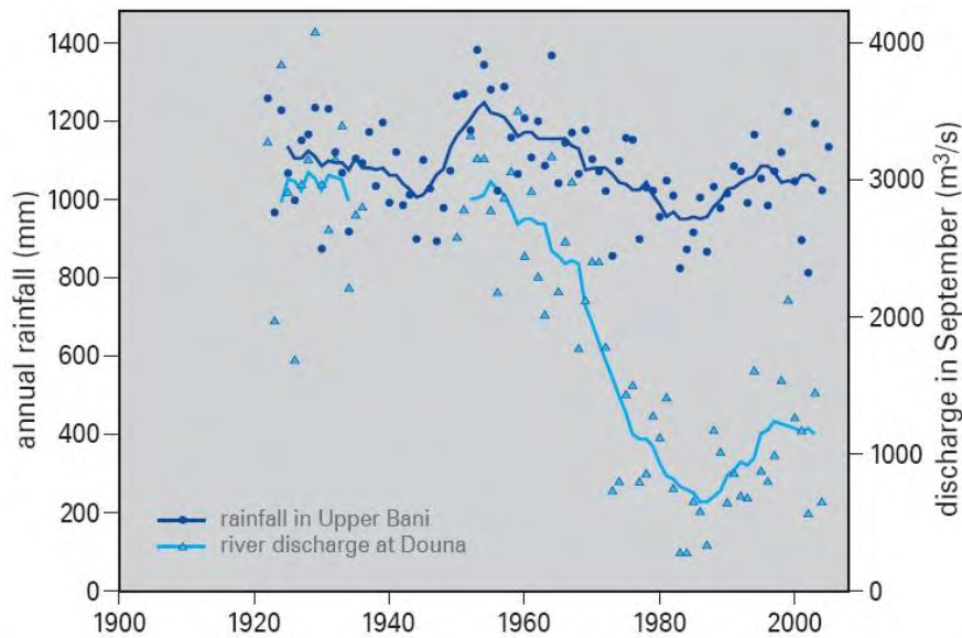
Figure 3-4- Annual rainfall of the Upper Bani averaged for 28 rainfall stations in the catchment area (dark blue symbols, left y-axis) and the river discharge in September at Douna (light blue symbols, right y-axis). The trends show 9-year running means. See Fig. 3.3 for the location of Douna and the rainfall stations. From: Zwarts et al. (2009).
