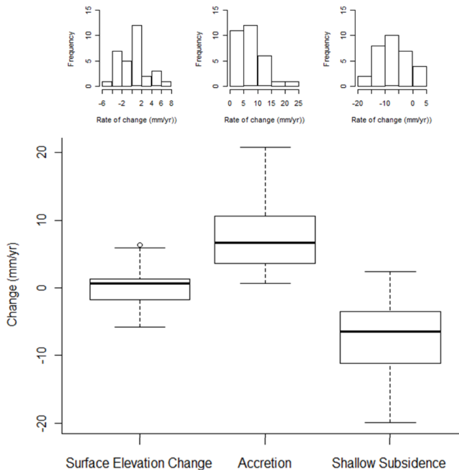
Figure 10. Rates of surface elevation change, accretion and shallow subsidence from the studies included in Table 2, with frequency histograms above the bars. Raw data and sources given in Appendix A; data now disaggregated within locations where these data are given in the source papers (e.g. surface elevation change was measured in 7 sites on Kosrae, Micronesia (Krauss et al. , 2010); the mean of these 7 measurements was used in Section 2.2 to allow comparisons with other locations where data had already been averaged in the source papers).
