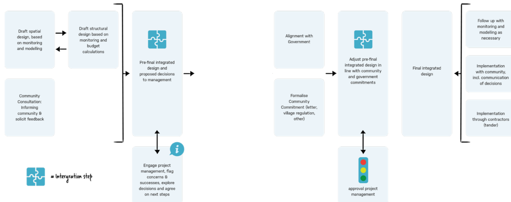
Figure 14. Process from design to construction for permeable structures © Wetlands International Indonesia
